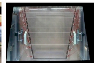
ALICE TPC upgrade
